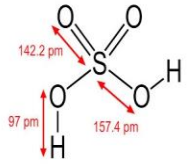
Sulfuric Acid (H 2 SO 4 )
